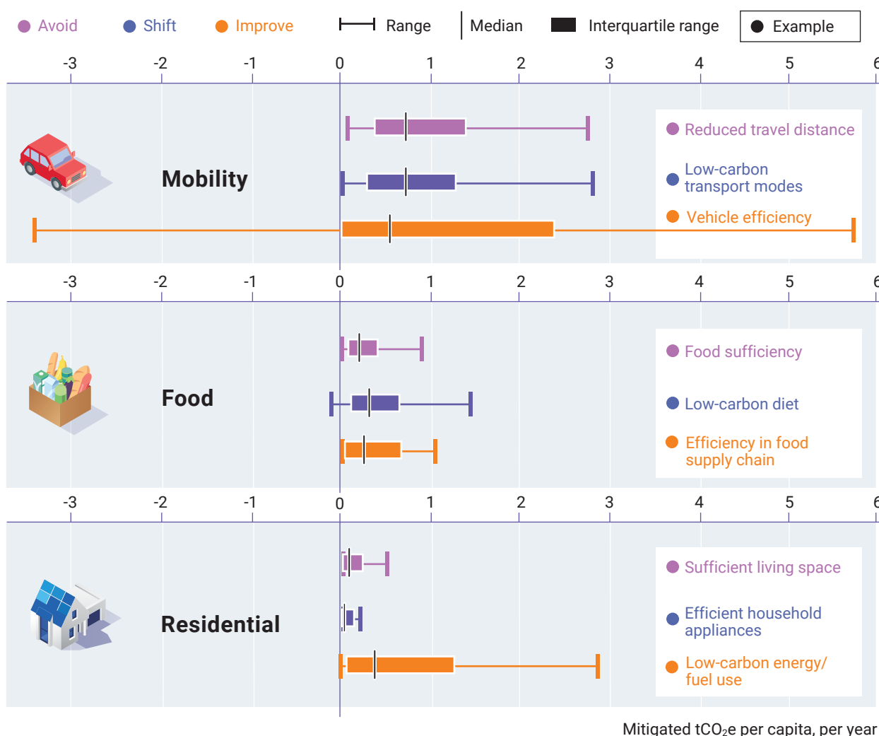
Figure 6.2. Carbon mitigation potential of Avoid, Shift and Improve consumption options within domains
